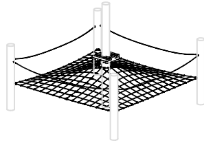
Horizontal Square Net with Centered Lookout
